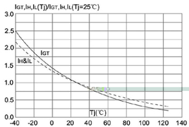
FIG.6: Relative indications of gate trigger current holding current and latching current versus junction temperature
